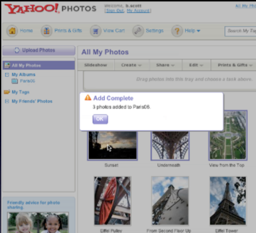
anti-pattern. y! photos. idiot boxes
